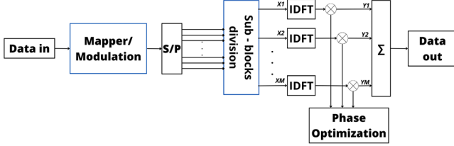
Fig. 6. Block diagram of OFDM transmitter with PTS.
