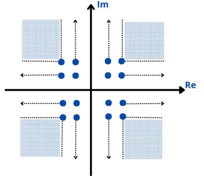
Fig. 12. ACE constellation for 16 QAM.
