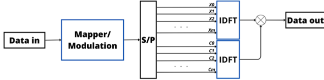
Fig. 11. Block diagram of OFDM transmitter for TI.
