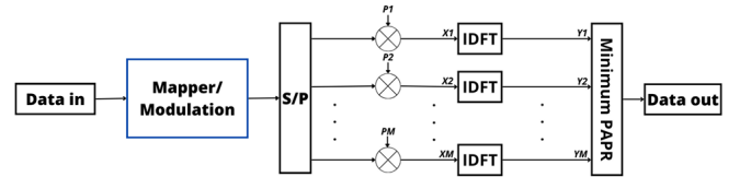
Fig. 7. Block diagram of OFDM transmitter with SLM.
