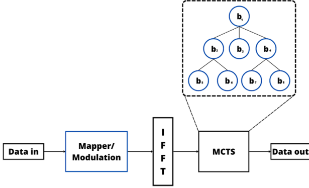
Fig. 15. Illustration of the MCTS transmitter.
