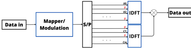
Fig. 10. Block diagram of OFDM transmitter for TR.
