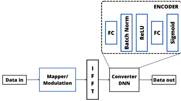
Fig. 14. Illustration of the DNN transmitter.
