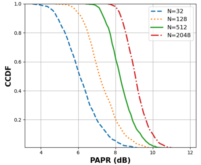
Fig. 5. CCDF of the PAPR for 32, 128, 512 and 2048 subcarriers.
