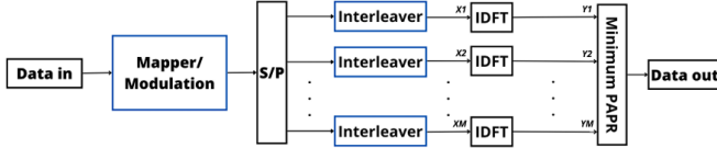
Fig. 8. Block diagram of OFDM transmitter with interleaving.
