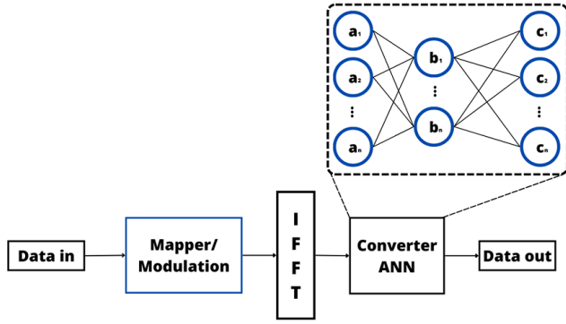
Fig. 13. Illustration of the ANN transmitter.
