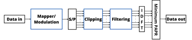
Fig. 9. Block diagram of OFDM transmitter with clipping and filtering.
