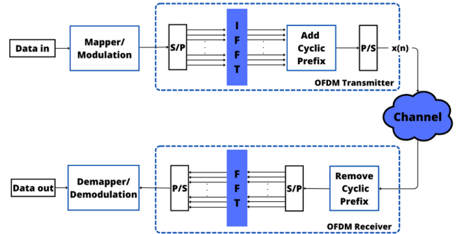
Fig. 4. Block diagram of a baseband OFDM system.
